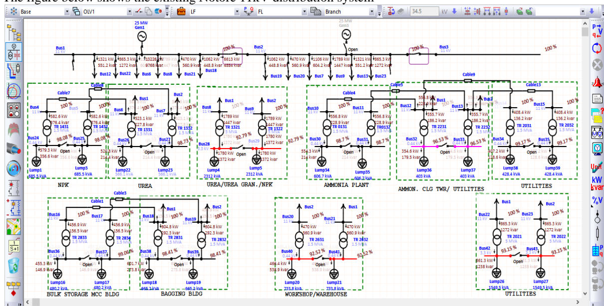
Figure 4.1: Existing Notore 11kV Distribution System
