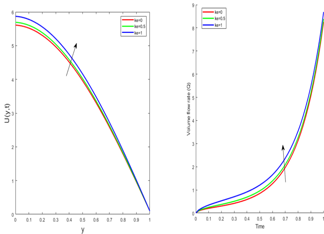
Figure 3: electric field effect on axial velocity and volumetric flow rate
