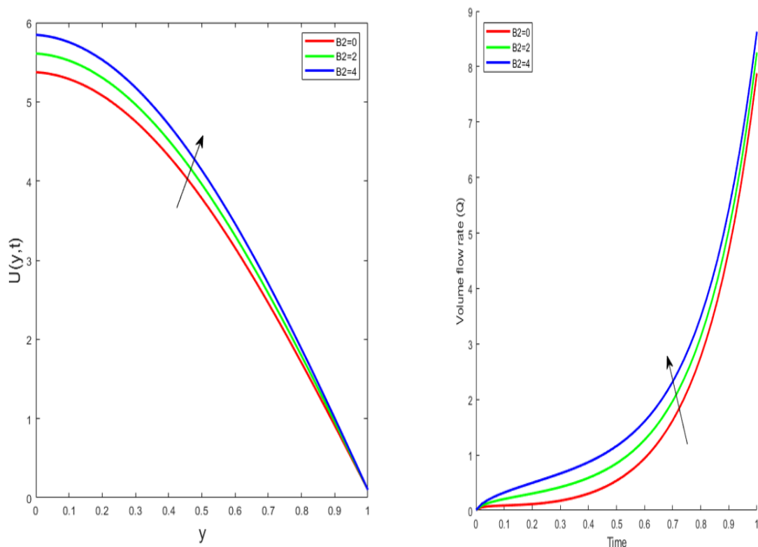
Figure 5; impact of body acceleration on axial velocity and volume flow rate
