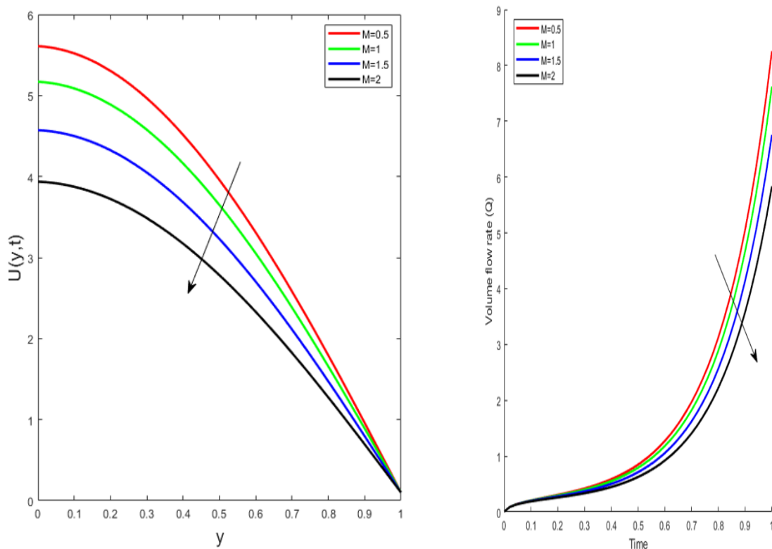
Figure 6; role of magnetic field on axial velocity and volume flow rate
