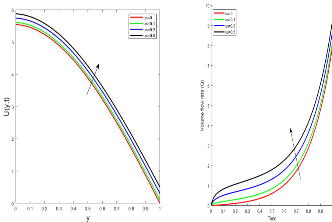
Figure 4; effect of slip parameter on axial velocity and volume flow rate
