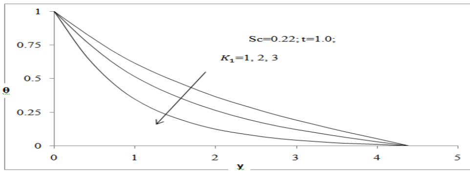
Fig.4 (d): Concentration Profile for different values of K_1
