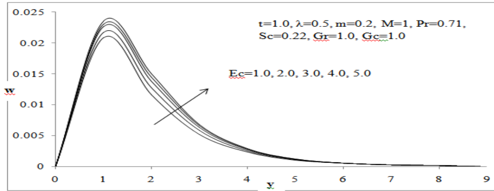
Fig.3 (b): The Secondary velocity profiles for different values of E_c
