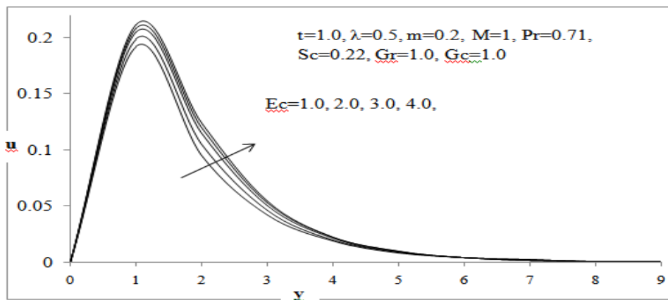
Fig.3 (a): The Primary velocity profiles for different values of Ec
