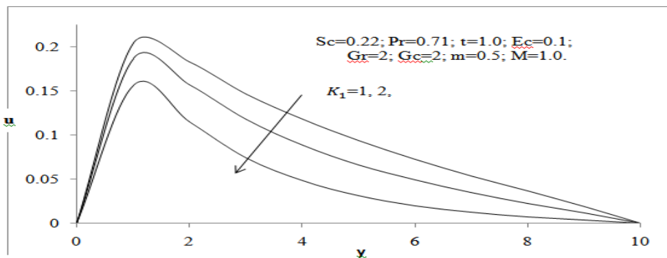
Fig.4 (b): The Secondary Velocity Profile for different values of K_1
