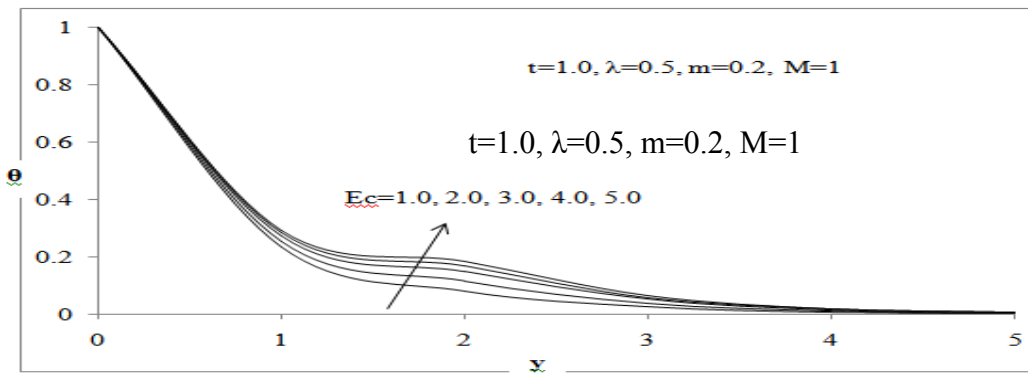
Fig.3 (c): Temperature Profiles for different values of E_c
