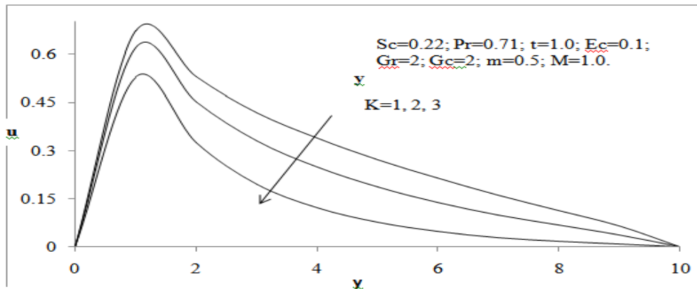
Fig.4 (a): The Primary Velocity Profile for different values of K_1
