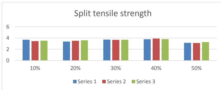
Split tensile strength test on 7days, 14days and 28 days
